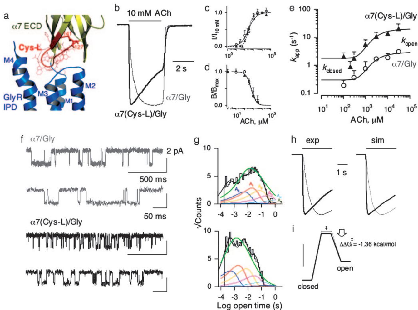
Fig. 2. Kinetic characterization of \alpha 7(\text{Cys-L})/\text{Gly} chimera. (a) 3D model of the \alpha 7/\text{Gly} interface (one subunit shown) with \alpha 7 ECD (pale yellow) and GlyR IPD (blue marine). \alpha 7 Cys-loop and numbers are highlighted in red. (b) Normalized whole-cell currents (10 mM ACh) through \alpha 7/\text{Gly} (gray trace) and \alpha 7(\text{Cys-L})/\text{Gly} (dark trace). (c) Dose-response curves for \alpha 7/\text{Gly} (open circles) and \alpha 7(\text{Cys-L})/\text{Gly} (filled triangles). Whole-cell currents are normalized to 10 mM ACh-evoked currents. (d) ACh competition against \alpha - ^{125}\text{I} -bungarotoxin binding to \alpha 7/\text{Gly} (open circles, K_p = 540 \mu\text{M} ) and \alpha 7(\text{Cys-L})/\text{Gly} (filled triangles, K_p = 600 \mu\text{M} ). Maximal binding ( B_{\text{max}} ) is defined without ACh. (e) Concentration dependency of k_{\text{app}} for \alpha 7/\text{Gly} (open circles) and \alpha 7(\text{Cys-L})/\text{Gly} (filled triangles). Data are fitted with Eq. 1. For \alpha 7/\text{Gly} , data are the same as for Fig. 1f. For clarity, only positive error bars are represented. (f) Single-channel currents through \alpha 7/\text{Gly} (gray trace) and \alpha 7(\text{Cys-L})/\text{Gly} (dark trace) from cell-attached patches (10 \mu\text{M} ACh). Currents are displayed at 1-kHz bandwidth, with channel openings as downward deflections. (g) Open time histograms. Simulated probability density functions are indicated for each unliganded ( A_0 ) and liganded open state ( A_1, \dots, A_5 ). The sum of these functions is indicated in green traces (for details, see Supporting Materials and Methods ). (h) Comparison of computed (sim) and experimental (exp) whole-cell currents (10 mM ACh) through \alpha 7/\text{Gly} (gray traces) and \alpha 7(\text{Cys-L})/\text{Gly} (dark traces). (i) Gating free energy diagram for \alpha 7/\text{Gly} (gray trace) and \alpha 7(\text{Cys-L})/\text{Gly} (dark trace). \Delta\Delta G^{\text{closed}} is arbitrarily set to zero, and vertical bar represents 10 kcal/mol.
