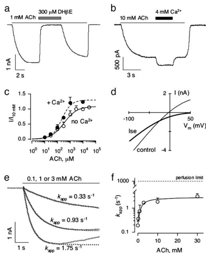
Fig. 1. Functional characterization of \alpha 7/\text{Gly} chimera. (a) Whole-cell current (1 mM ACh) through \alpha 7/\text{Gly} and its reversible inhibition by 300 \mu\text{M} dihydro- \beta -erythroidine (DH \beta E). (b) Current potentiation by 4 \text{ mM Ca}^{2+} during a 10\text{-mM} ACh application. Recorded from a different cell. (c) Dose-response curves in the absence (open circles) or presence (filled circles) of 4 \text{ mM Ca}^{2+} . Currents are normalized to 10 \text{ mM} ACh-evoked currents. (d) Current-voltage relationships. External sodium chloride (control condition) substituted by sodium isethionate (Ise condition). (e) Typical currents evoked by 100 \mu\text{M} (bottom trace), 1 \text{ mM} (middle trace), or 3 \text{ mM} (top trace) ACh concentrations. k_{app} , derived from single exponential functions, are indicated. (f) k_{app} plotted as function of ACh concentrations. Data were fitted with Eq. 1. For clarity, only positive error bars are represented.
