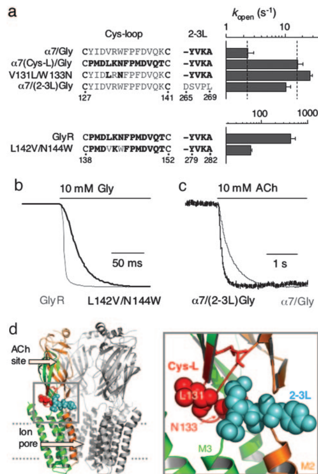
Fig. 3. Tuning the activation kinetics in LGICs. (a) k_{open} bar plot of the indicated constructions. Sequences of the Cys-loop and 2-3L region are indicated. Residues from \alpha 7 nAChR are indicated in gray and GlyR in bold-type characters. (b) Normalized whole-cell currents (10 mM glycine) through GlyR WT (gray trace) and L142V/N144W mutant (dark trace). (c) Normalized whole-cell currents (10 mM ACh) through \alpha 7 /Gly (gray trace) and \alpha 7 /(2-3L)Gly (dark trace). (d) Mapping of the identified residues on the \alpha 7 /Gly 3D model (red spheres for Cys-L and cyan for 2-3L). The inner and outer blocks are colored in orange and green, respectively. For clarity, only four subunits are represented. (Inset) Enlarged view of the coupling zone.
